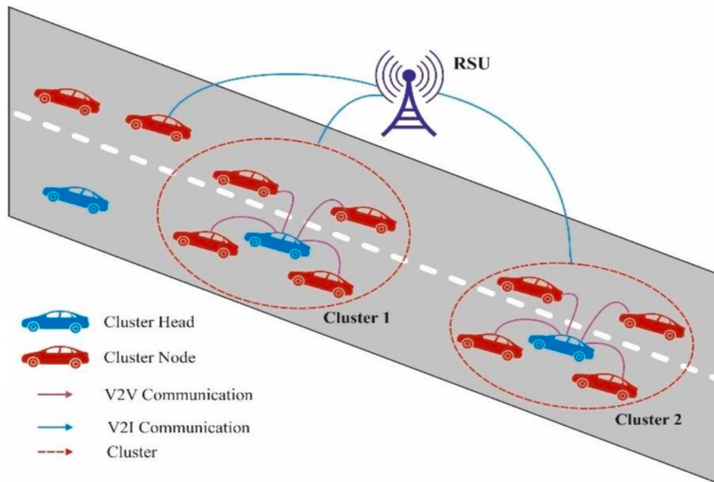
Fig. 7. Clusters division [61].
