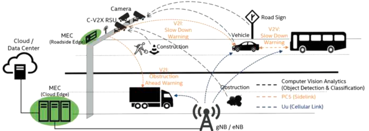
Fig. 5. Vehicle To Roadside Units (V2R) [42].
