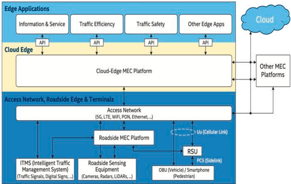
Fig. 4. Implementation of C-V2X services on MEC platforms [42].
